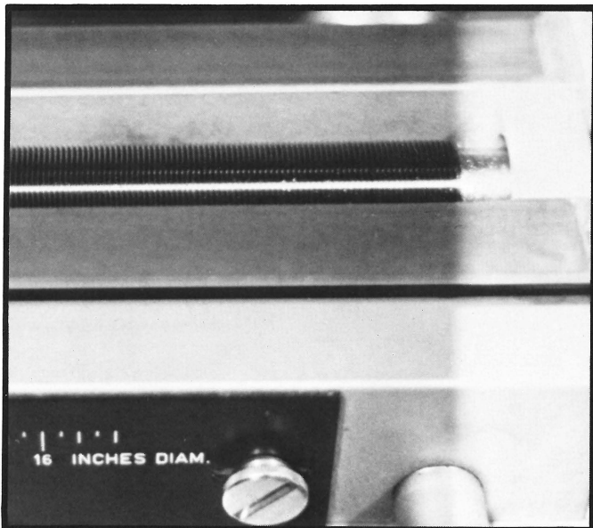
The lead screw of a Neumann Lathe. The carriage rides on this screw on its journey across the disc. The "pitch" is changed by speeding up or slowing down the motor which turns it.
