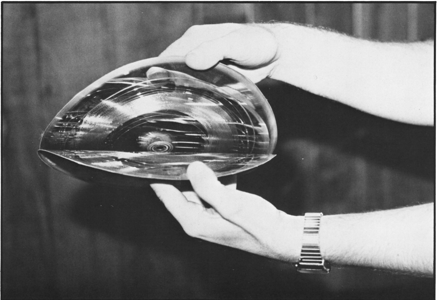
Separating the metal master and the mother.
