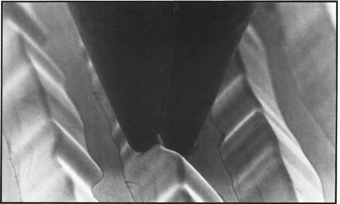
This special stylus plays only stampers and metal mothers. As can be seen in this remarkable photo, it straddles the negative groove.
