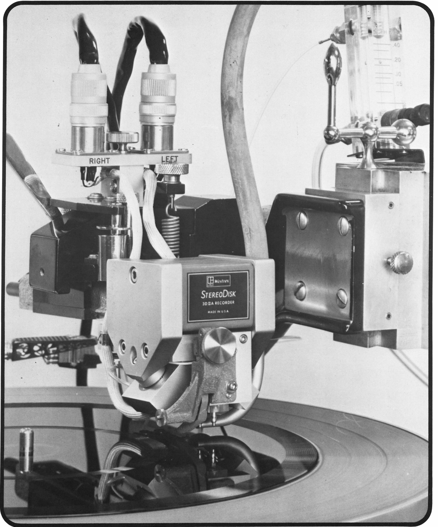
The Westrex 3DII AH Stereo Cutterhead. (Manufacturer's photo)
