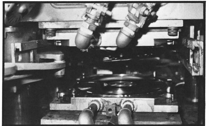
A stamper mounted in a record press.
