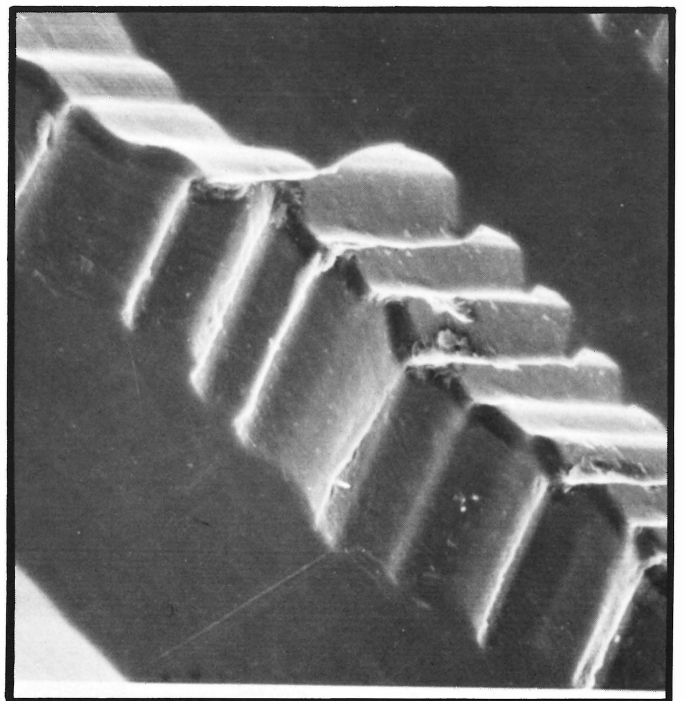
This photo shows the raised grooves of a metal master. The debris to be removed by de-ticking are clearly visible. (Photo courtesy of Stanton Magnetics)
