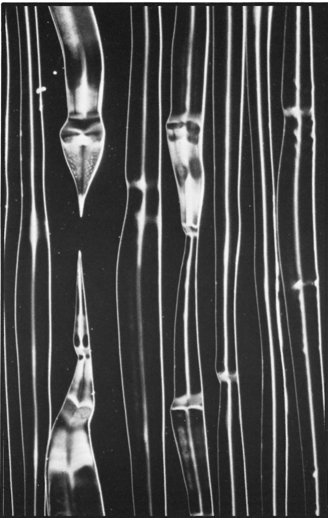
Out of phase material can make a cutterhead "lift out," thereby breaking the groove. The lift out shown here is unacceptable.
