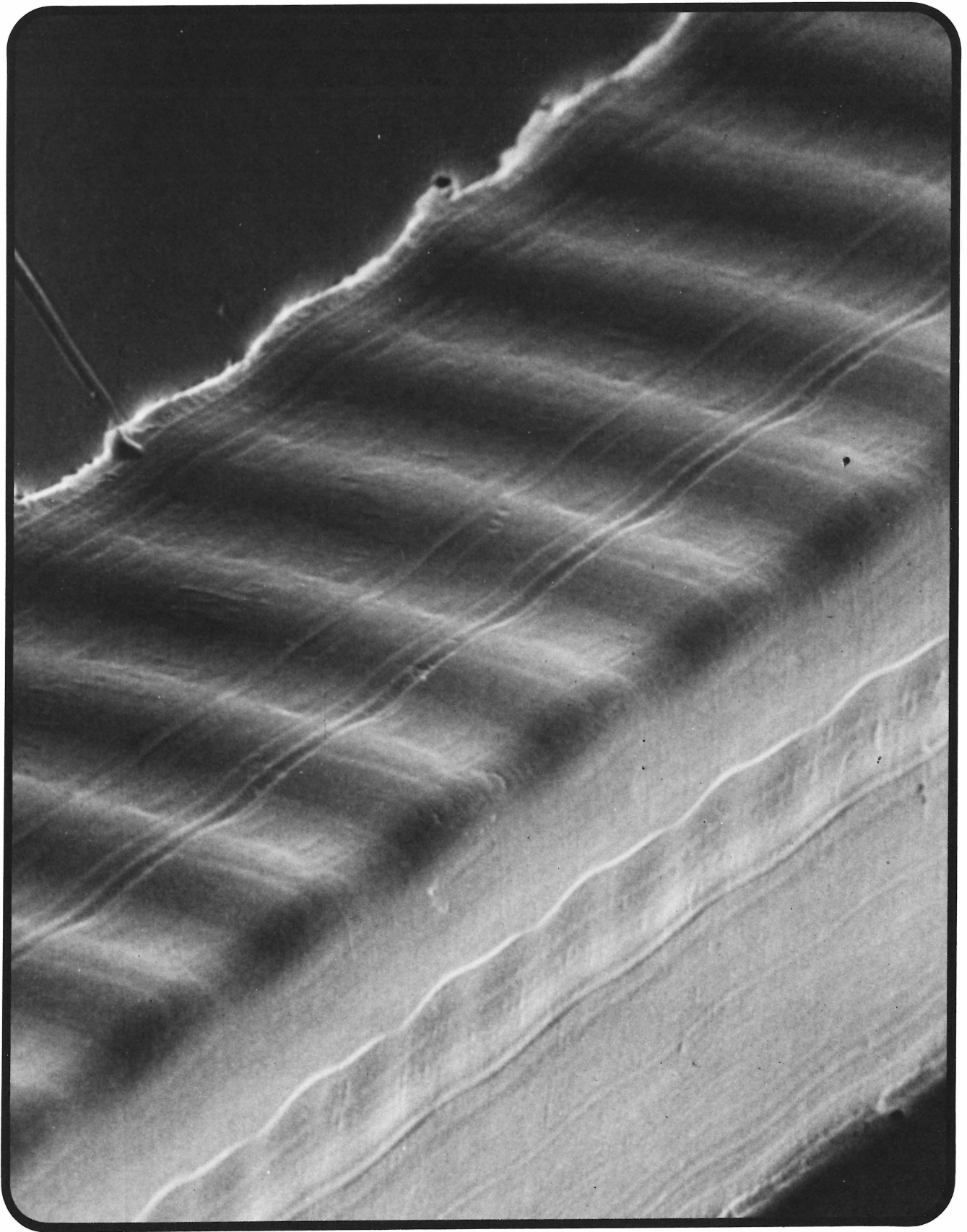
A test record after 100 plays. Note 20KHZ modulation on right groove wall, none on left (10,000 magnification). Groove wear is clearly evident. (Photo courtesy of Stanton Magnetic)
