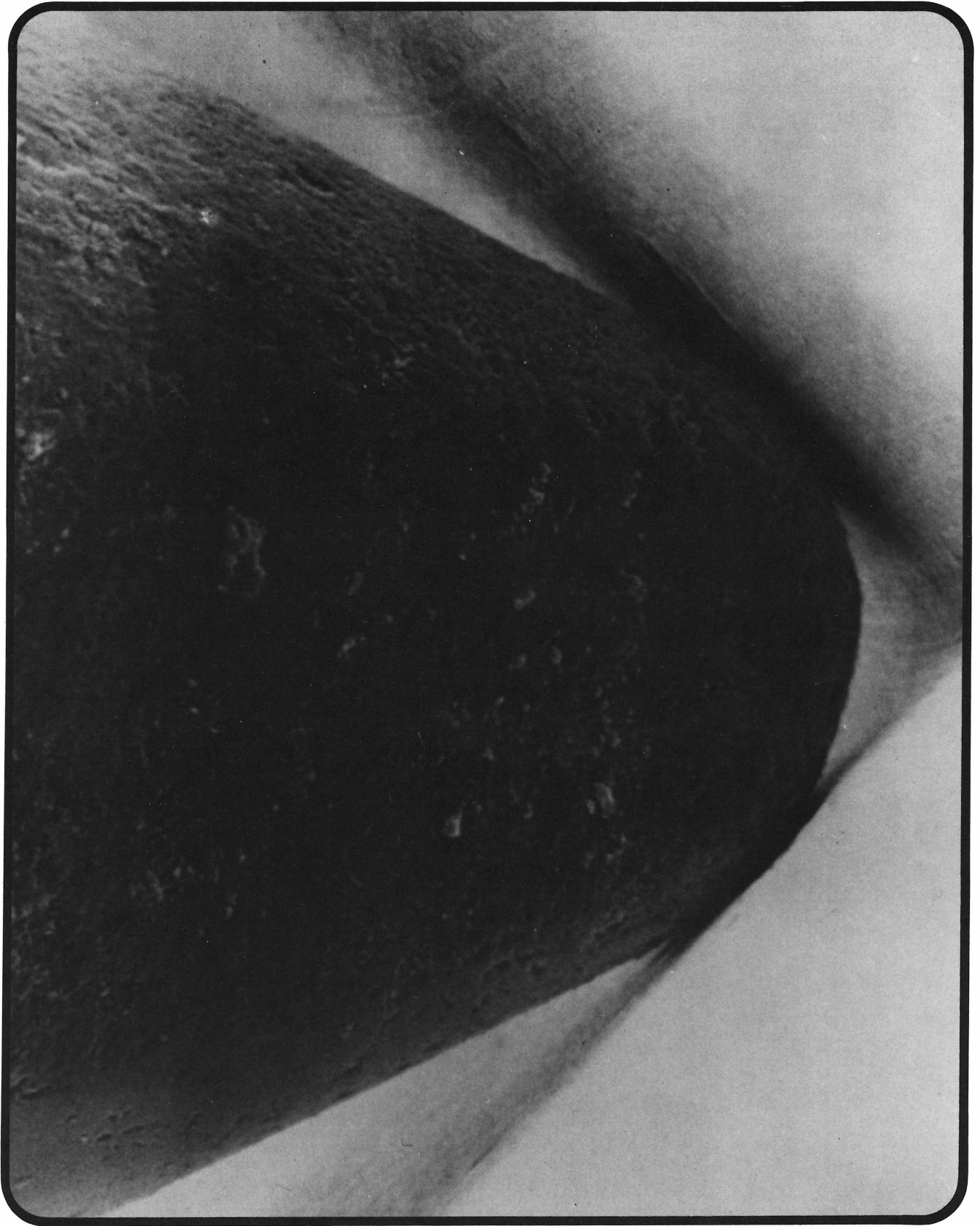
A spherical playback stylus resting in a record groove in playing position (10,000 magnification). (Photo courtesy Stanton Magnetics)
