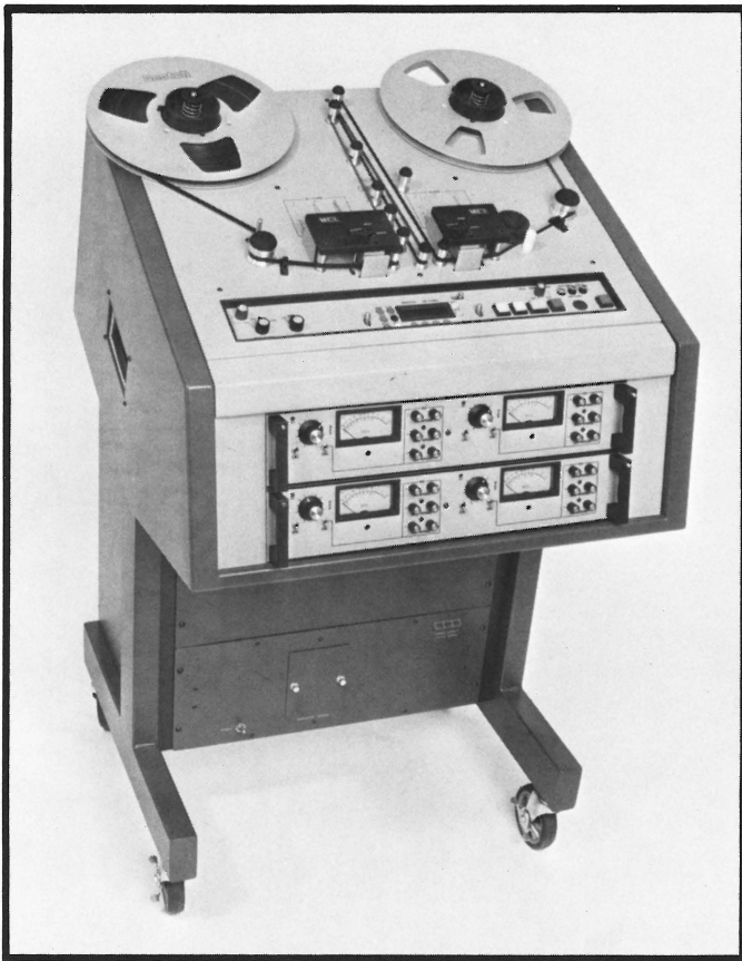
A disc mastering tape playback unit manufactured by MCI. Note long delay path between program and preview heads. (Manufacturer's photo)
