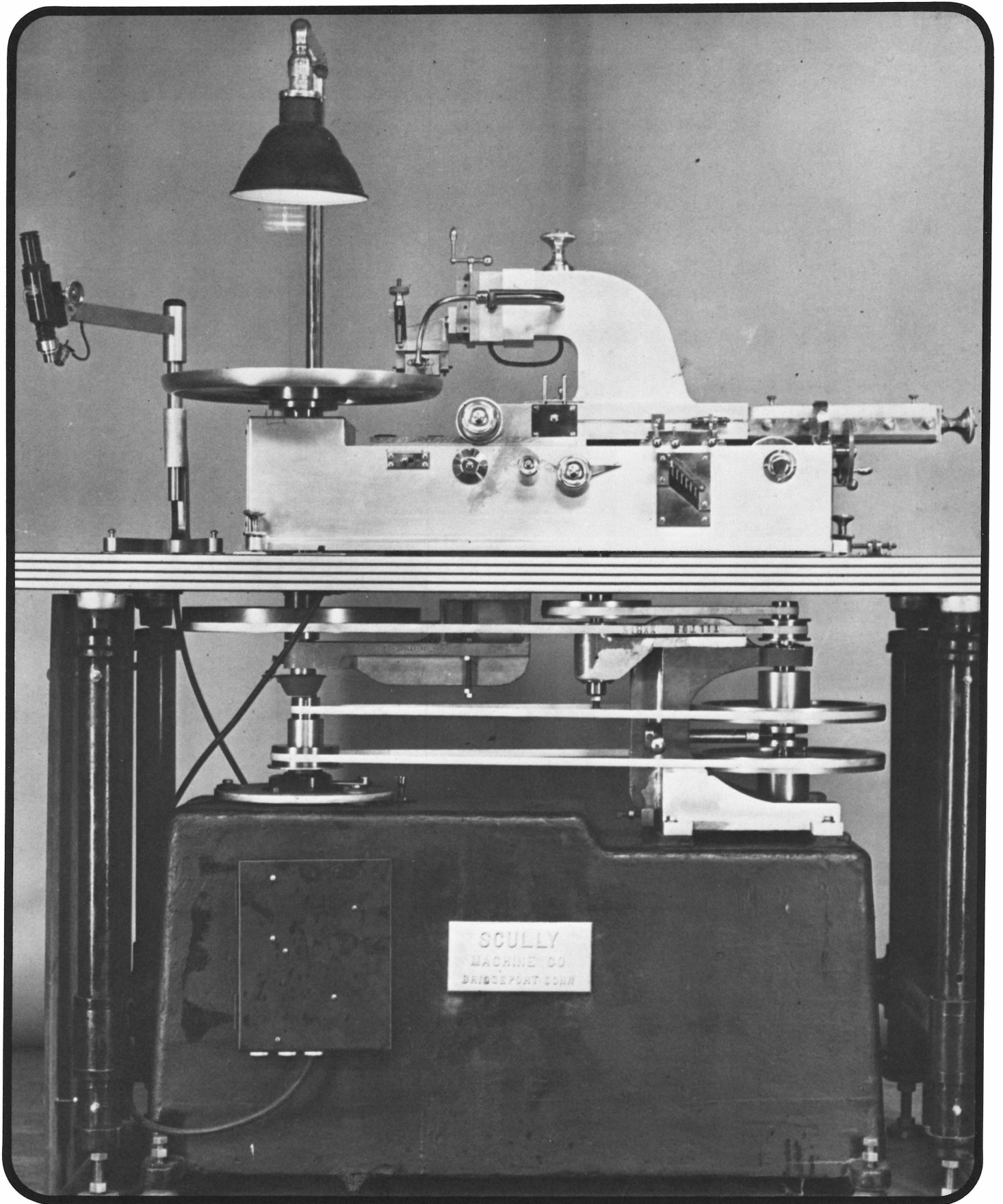
An old Scully Lathe, with covers removed to show the drive system. Over 600 were made. Many are still in use. (Manufacturer's photo)
