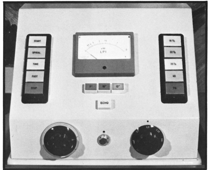
Control Section of a Neumann Lathe, showing turntable speed indicator, lathe function control and L.P.I. Meter.
