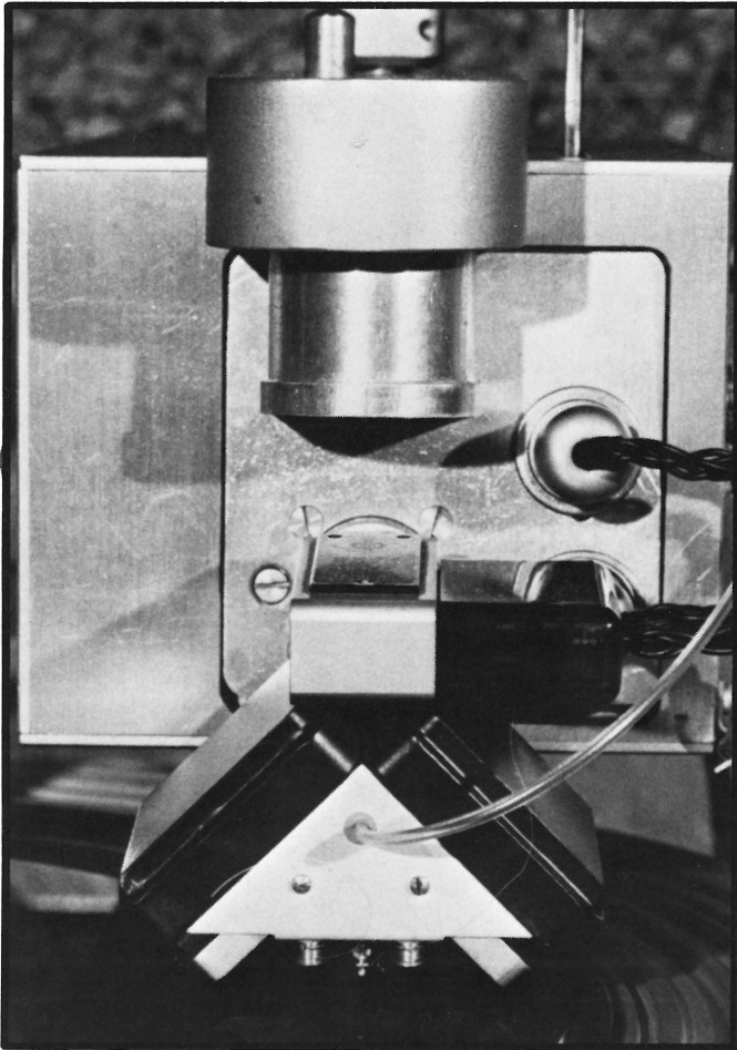
The Neumann SX-74 Stereo Cutterhead.
