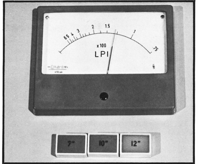
The LPI Meter shows our cutting pitch. Here, 130 L.P.I.
