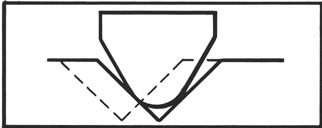
Cross section of a cutting stylus cutting a mono groove, showing the plane of modulation.
