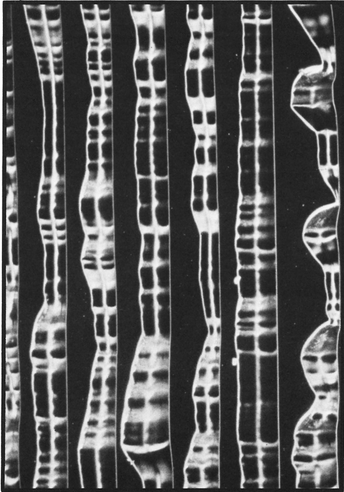
Picture of stereo grooves with information on left channel only.
