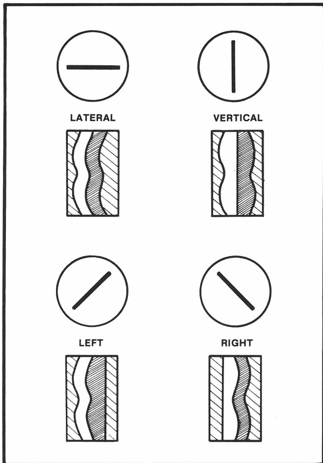
Oscilloscope patterns with matching groove types.
