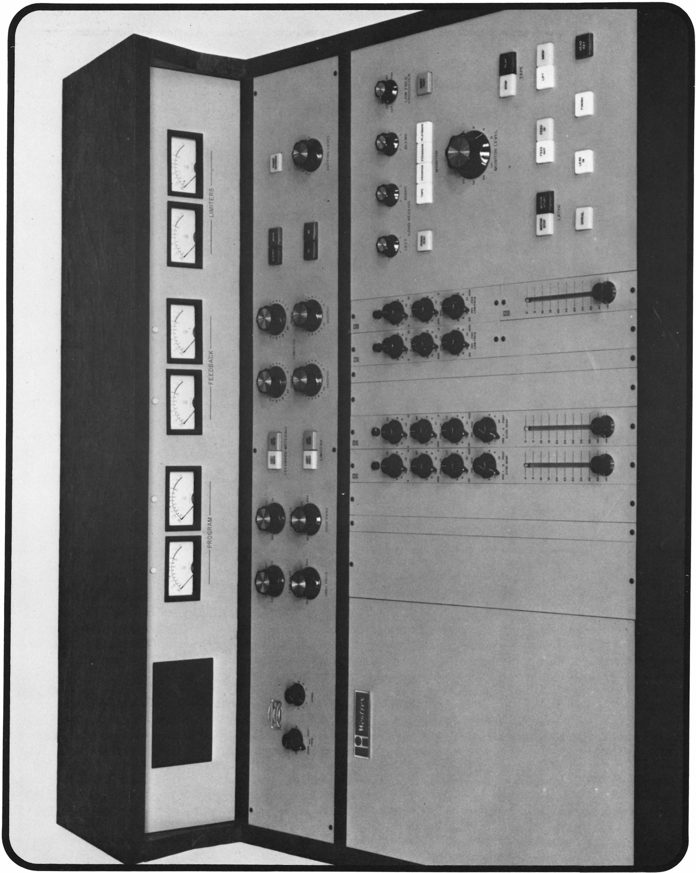
The Westrex Mastering Console. (Manufacturer's photo)
