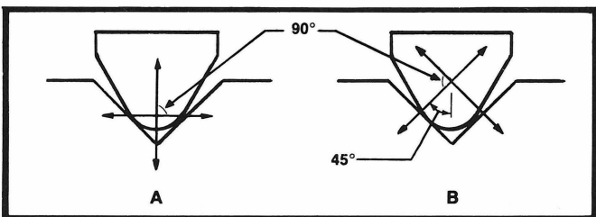
Technique A is the obvious way to cut two channels in a single groove. This method is extremely difficult.
