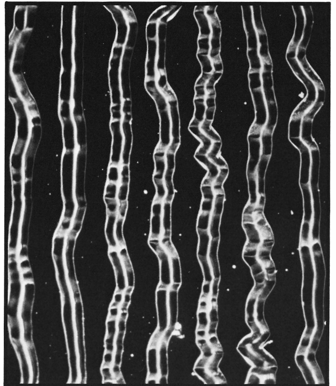
Acceptable high level cut.
