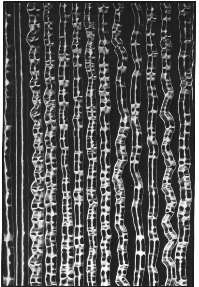
Variable pitch at work, controlling groove spacing to avoid overcut.
