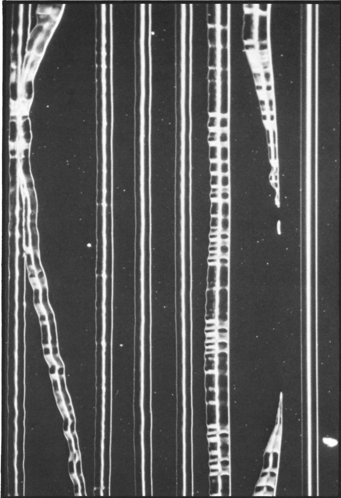
Overcuts, lift-outs and proper groove depth can be seen through the microscope.
