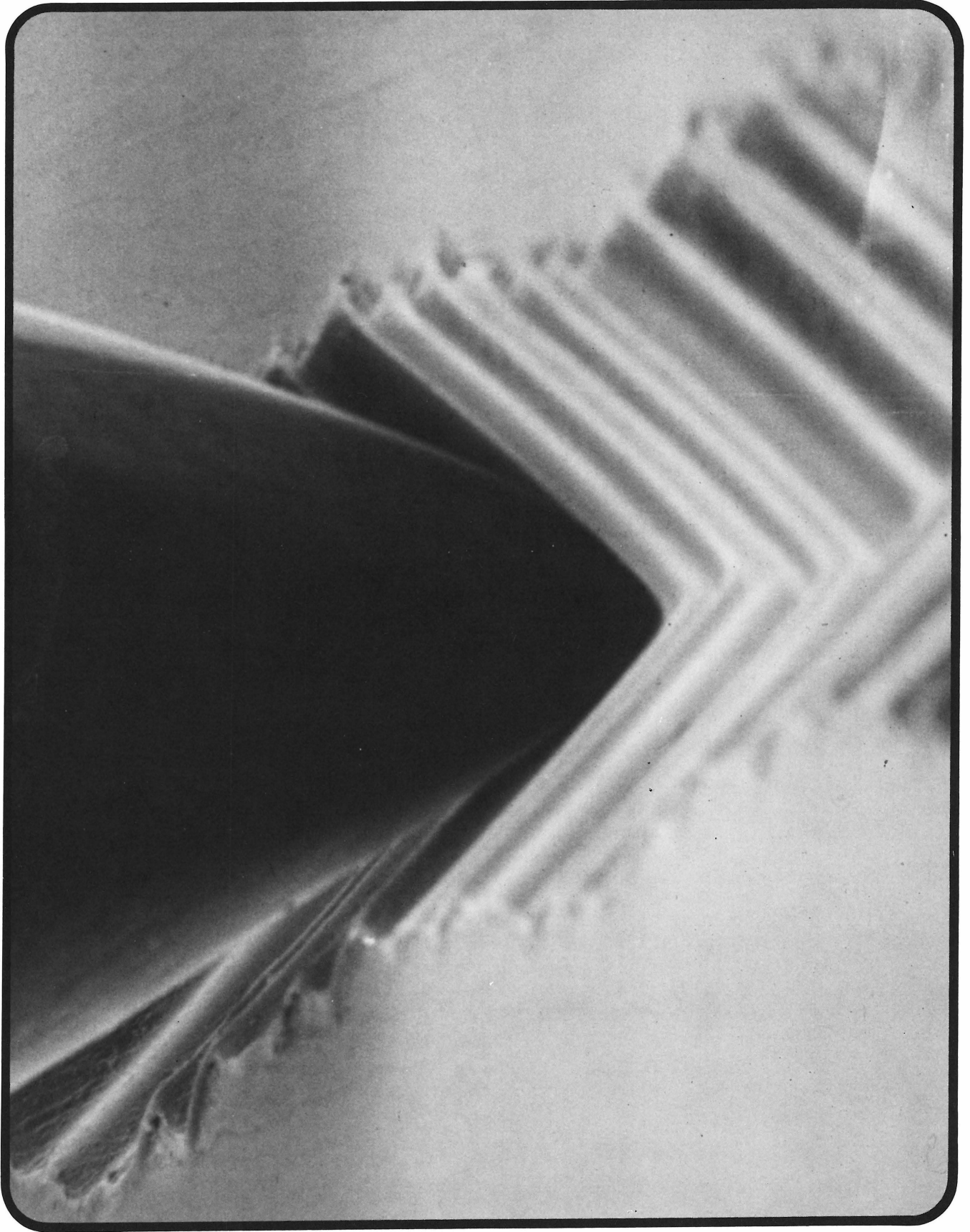
This photo shows just how hard a task the playback stylus has. Failure to completely trace out each and every groove undulation will result in distortion (1,000 magnification). (Photo courtesy of Stanton Magnetics)
