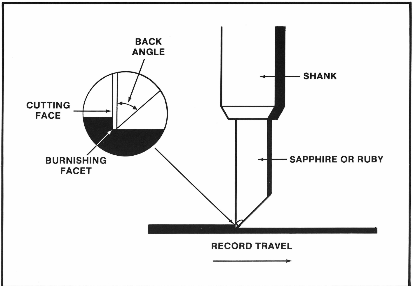
Enlarged view of stylus tip.
