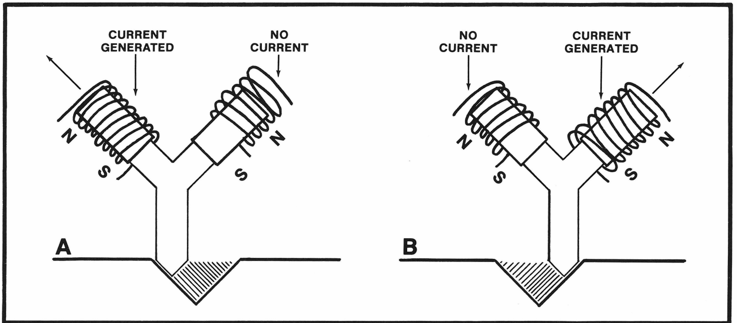
A playback stylus translates the stereo groove back into two distinct signals. "A" shows right channel output; "B" shows left channel output.
