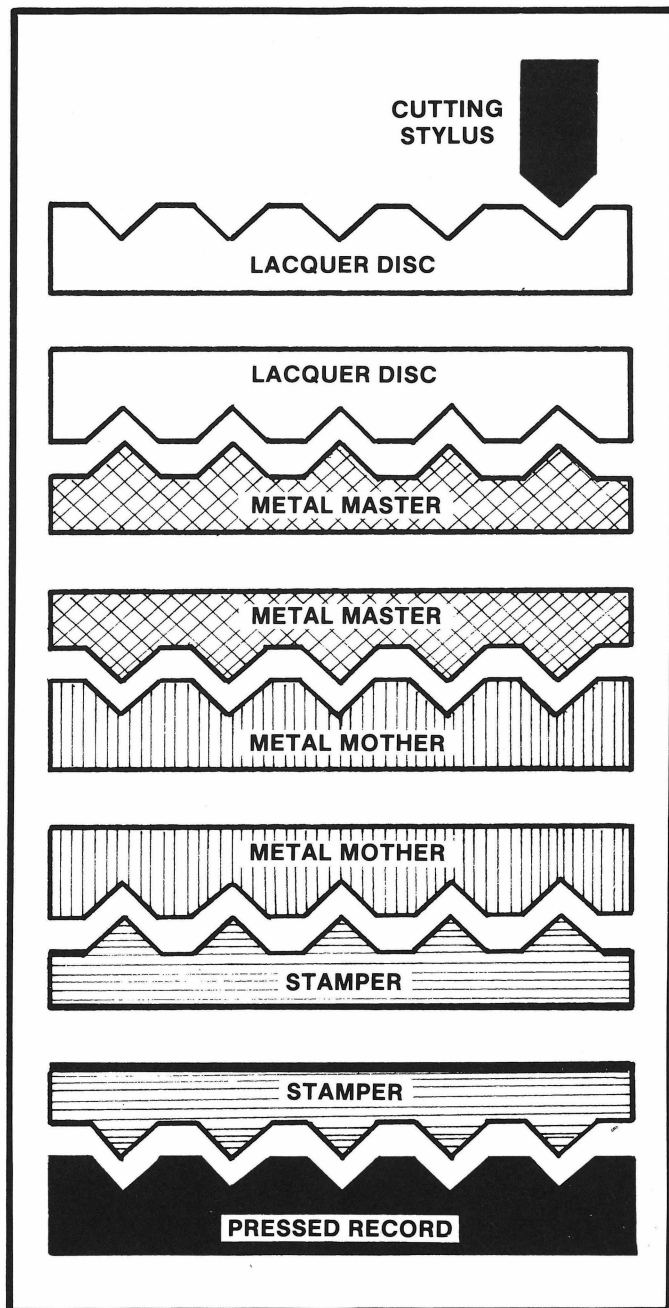
The various stages in the pressing process. Noise and other flaws can be introduced at any stage.
