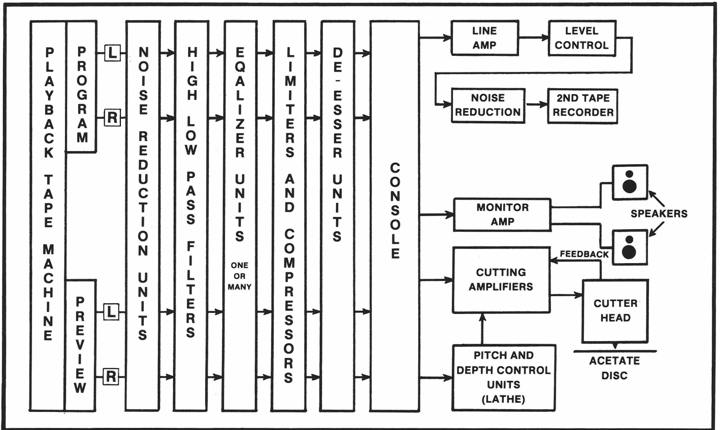
Simplified Flow Chart of a typical mastering chain.
