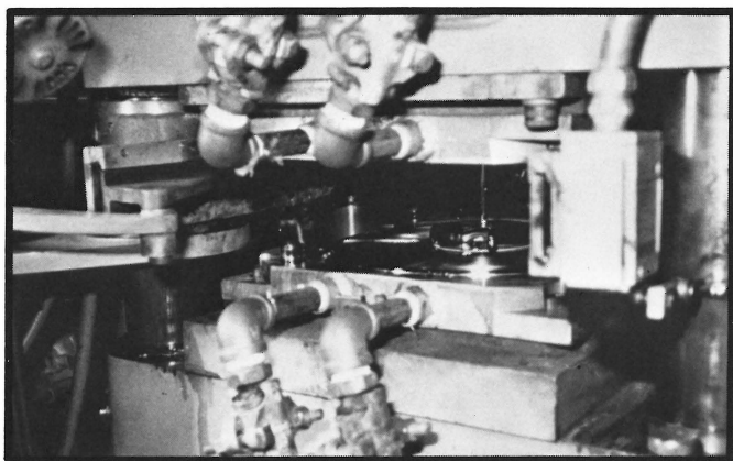
The warm vinyl biscuit in place in the center of the stamper.
