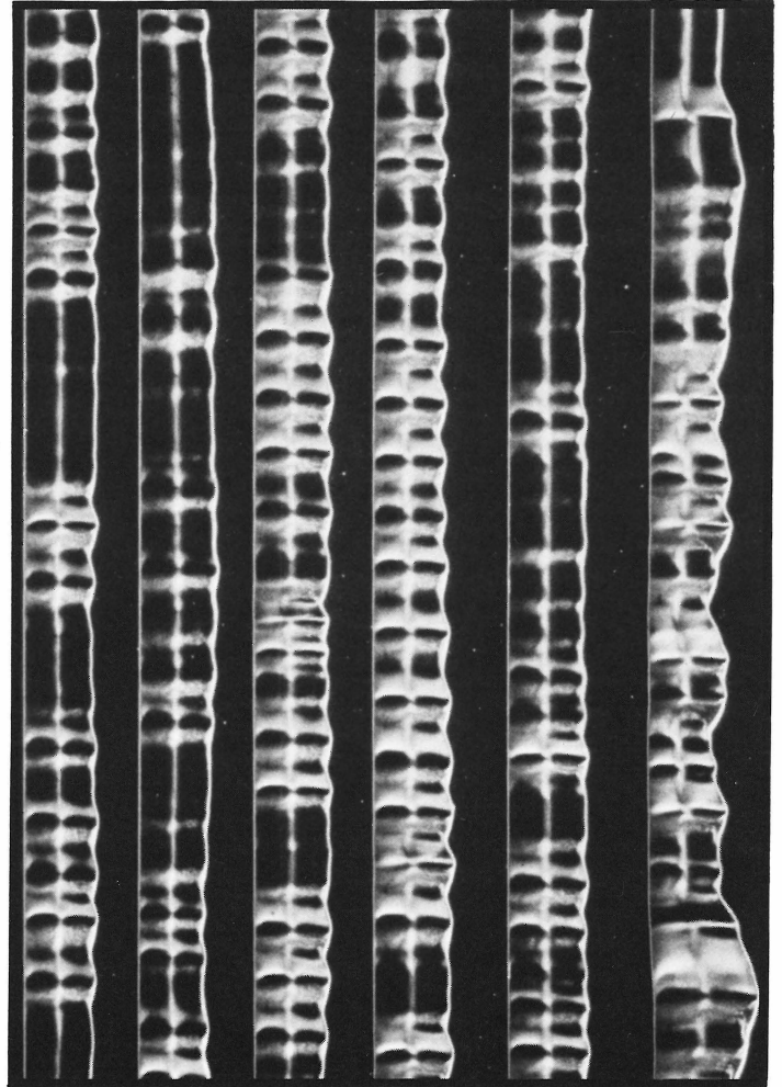
Picture of stereo grooves with information on right channel only.
