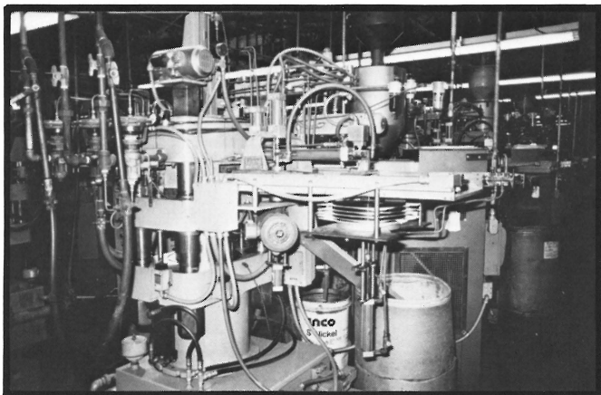
A modern, automated record press.
