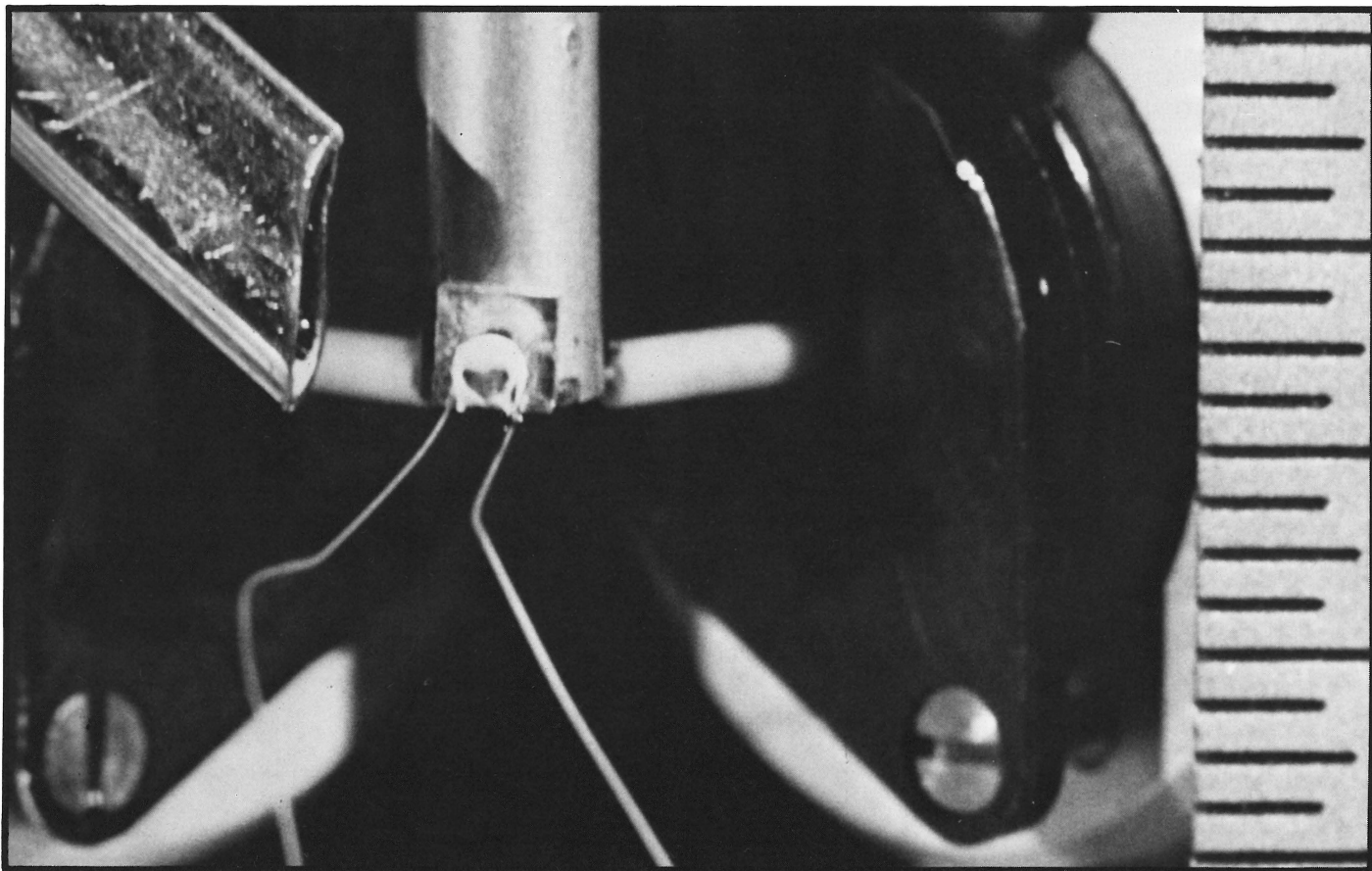
The cutting stylus mounted in the cutterhead. Note chip removal tube at left and the two heating wires.
