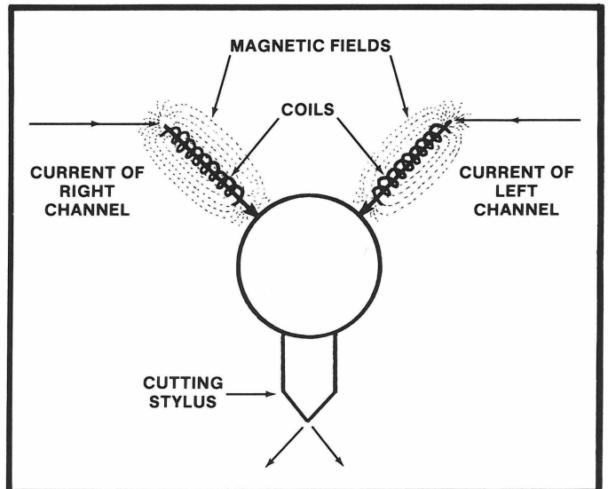
Simplified view of a stereo cutterhead.
